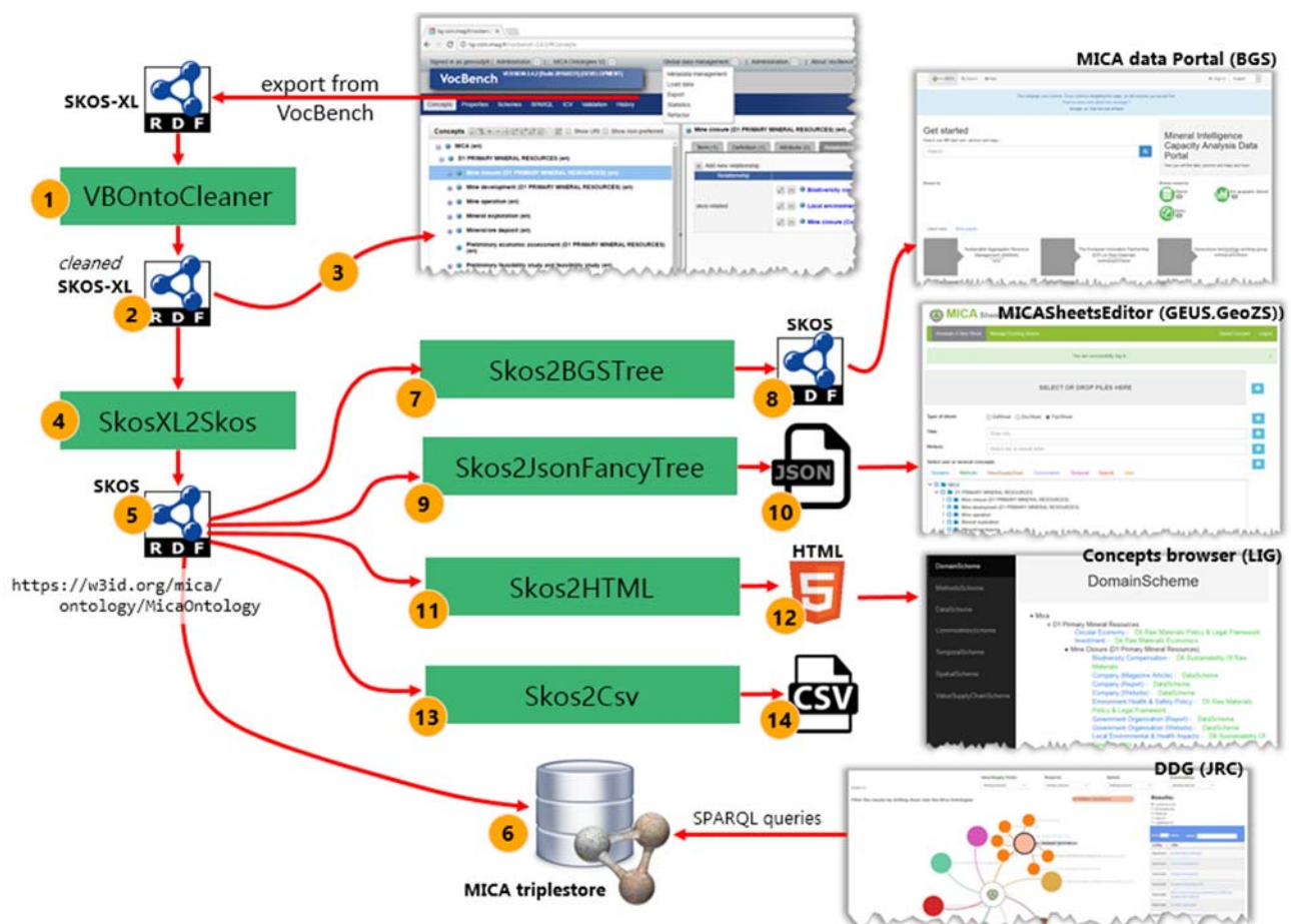
Figure 17 Management tools for the MICA Ontology.
