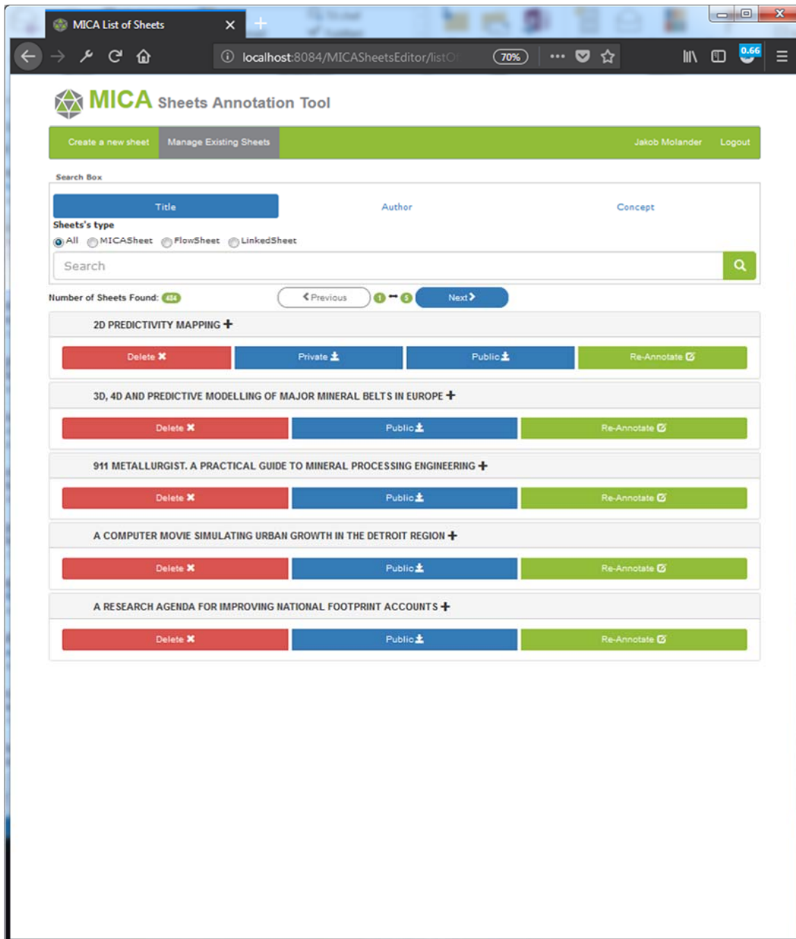
Figure 11 Search existing sheets.
