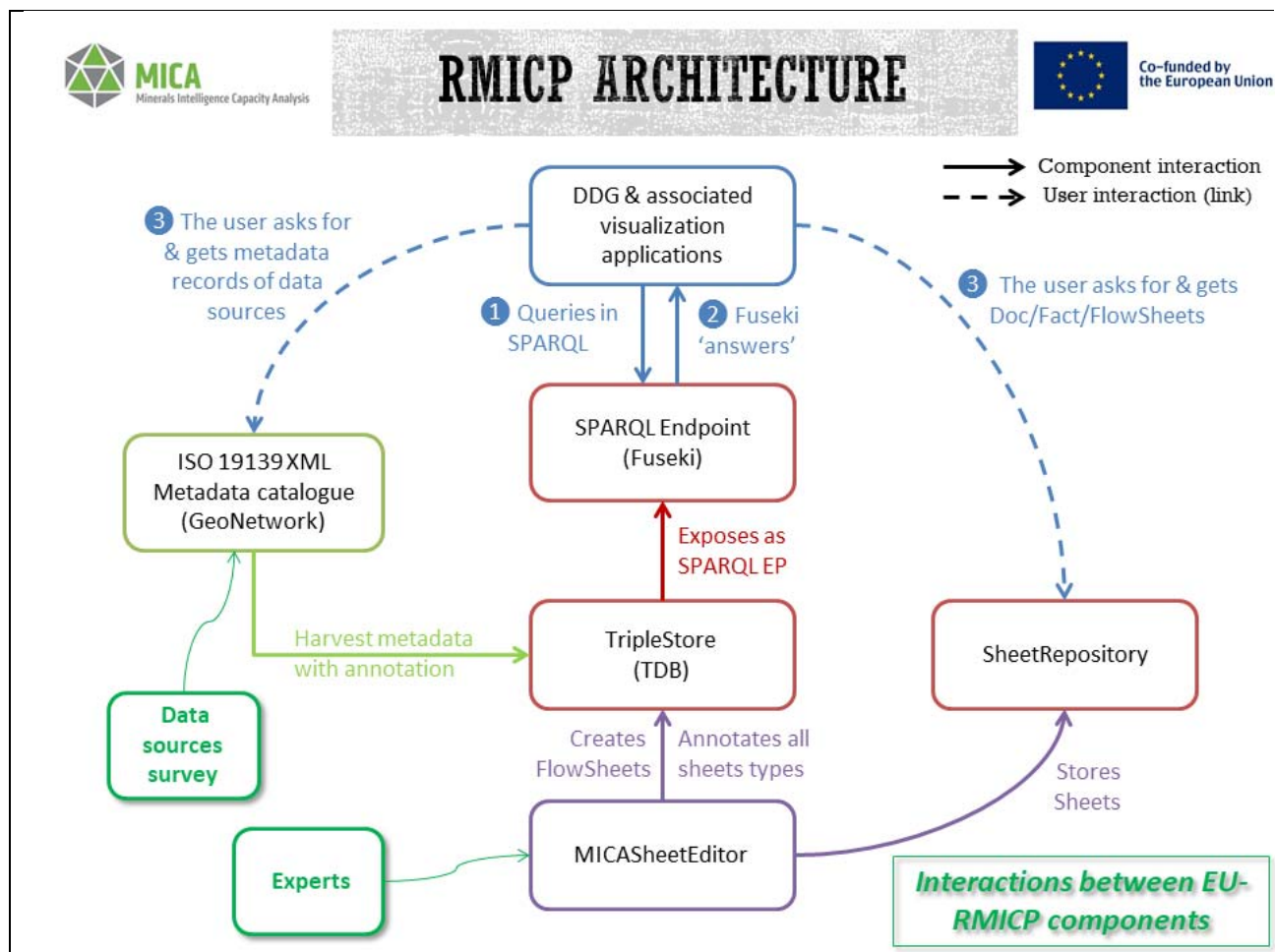
Figure 5 Interactions between the EU-RMICP components.
