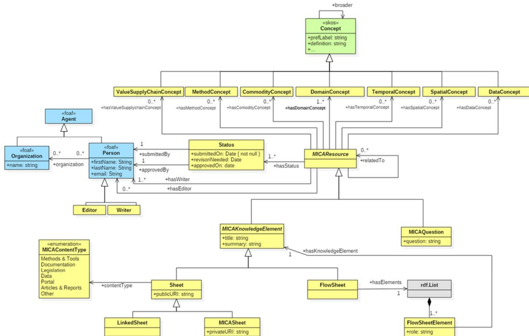
Figure 23 UML diagram class of MICA data model.
